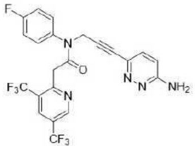
RP-6685 HNMR CDCl 3
